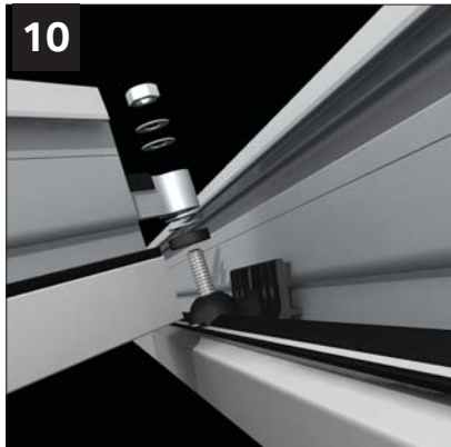
10 Now fit the jack rafters. The 2 part jack rafter kit is already fitted to the hip and jack rafter. Ease back the jack rafter undercladding. Each jack rafter kit is supplied with a number of washers. Trial fit the jack rafter and check that the glazing platforms are level. Adjust if necessary by adding or removing washers between the two part connecting kit, then tighten the nut. NOTE: If aluminium internal claddings are being used, fit hip internal cladding prior to fitting jack rafters.
