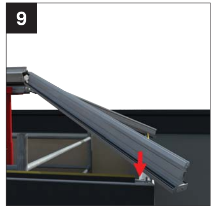
9 Remove nuts on eaves beam. Fit hip bars onto bolts at eaves end and hand tighten nuts.
