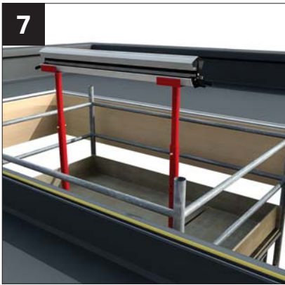
7 Prop ridge in position using suitable supports, centralising between eaves beam sections. (When the ridge features aluminium painted internal finish it will need to be protected whilst supporting).
