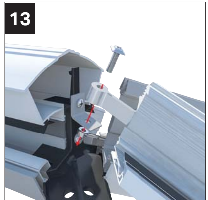
13 When a transom is fitted between hips, lift transom bar sleeved spiggot over bolt, then tighten nut.
